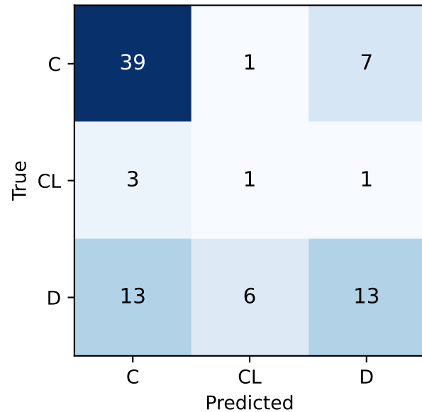
Naive Bayes (test)
