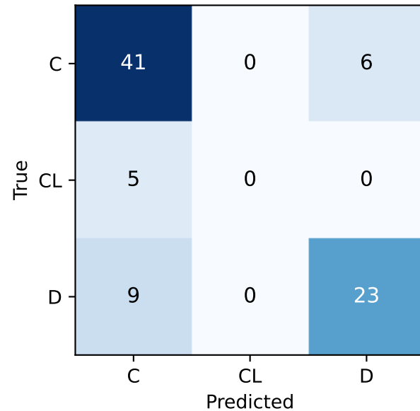
Random Forest (test)
